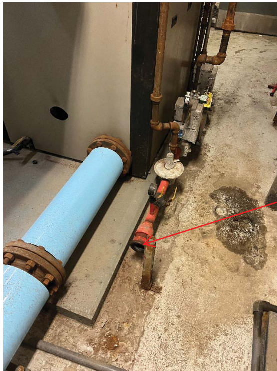
Photo No. 2 - U7 Grit and Screening Boiler No. 1 Disconnected Natural Gas Piping
